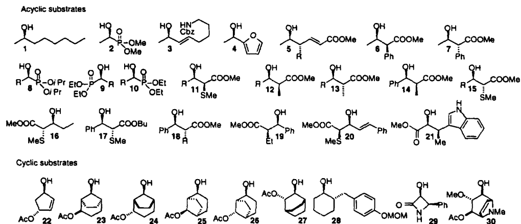
Figure 2. Examples from the literature of secondary alcohols resolved or desymmetrized by ANL. Structures show the fast reacting alcohol enantiomer. Most examples follow the rule in Figure 1. Details in Table 1.
