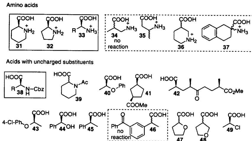
Figure 3. Carboxylic acids tested in enantioselective reactions with ANL. Enantioselectivities are moderate or better ( E > 10 ) only for the examples in the solid-line boxes. Examples in the dotted-line boxes did not react with ANL. Structures show the fast reacting enantiomer where the absolute configuration is known. Table 2 provides details for the examples from the literature and Table 3 lists experimental results for examples reported in this paper.
