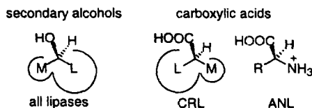
Figure 1. Empirical rules that predict the fast-reacting enantiomer in lipase-catalyzed reactions. For secondary alcohols, all lipases, including ANL, follow a rule that compares the size of the substituents at the stereocenter. For carboxylic acids, a rule based upon the size of the substituents at the stereocenter works for CRL, but not for ANL. A rule for ANL includes only \alpha -amino acids (including cyclic amino acids) and suggests that a charged \alpha -amino group is essential for high enantioselectivity. ANL always hydrolyzes the natural L-enantiomer. M represents a medium sized substituent, e.g., \text{CH}_3 ; L represents a large substituent, e.g., Ph; R represents any alkyl or aryl group.
